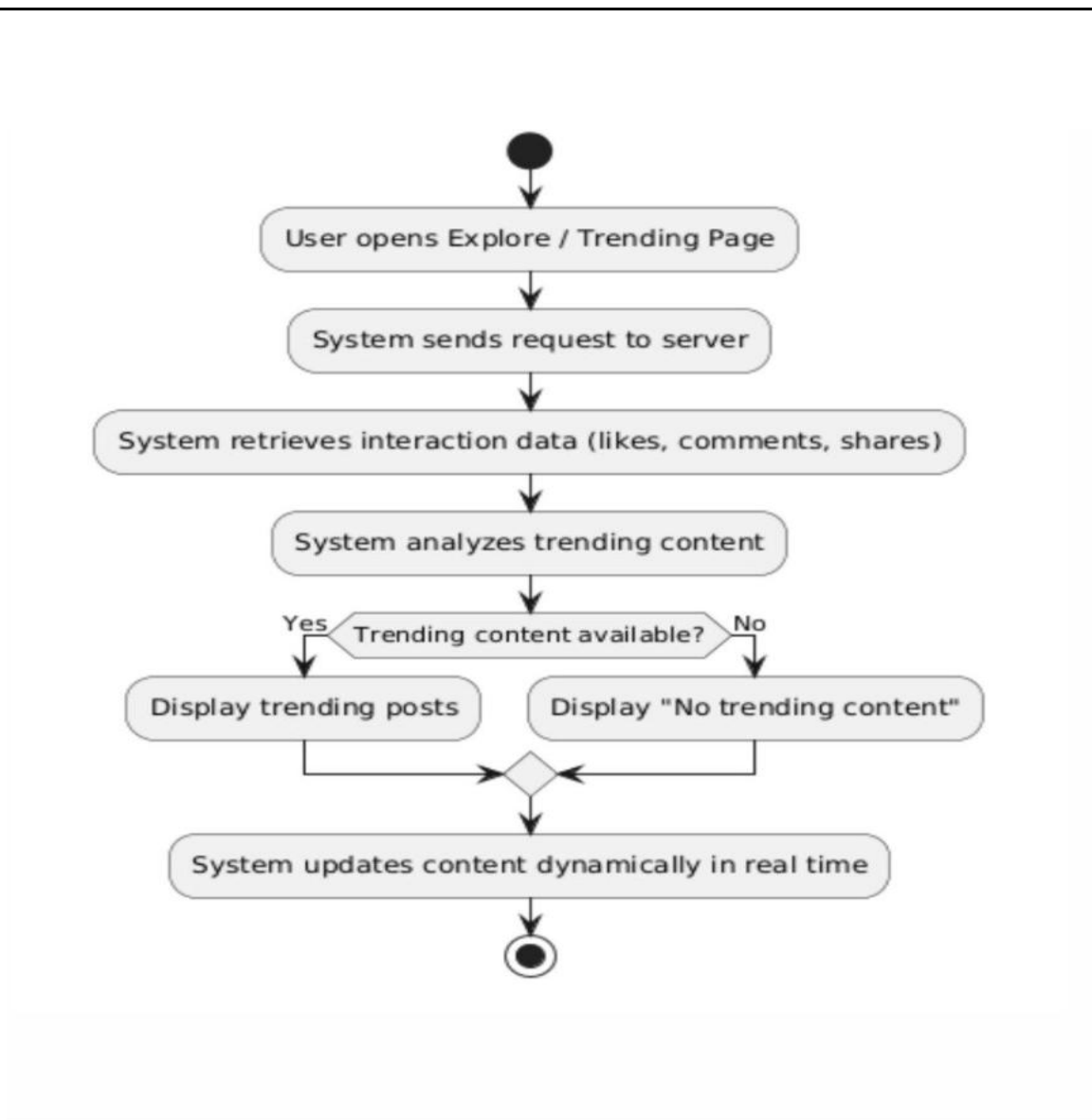
Figure 2.43: Activity Diagram Discover Trending Content in Real Time
