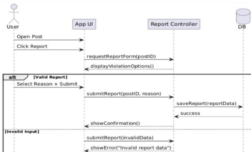
Figure 2.40: Sequence Diagram Report Inappropriate or Violating Posts
