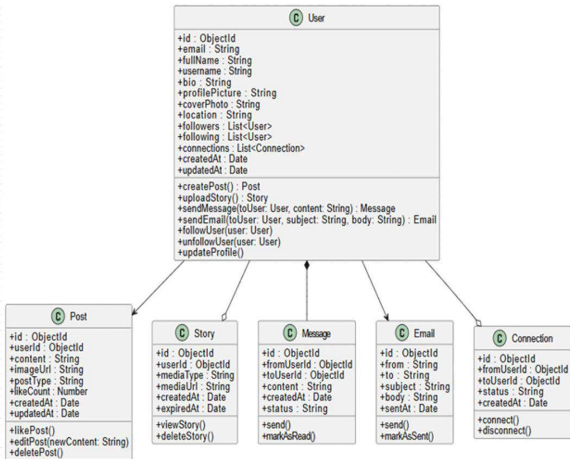
Figure 3.47: Class Diagram
