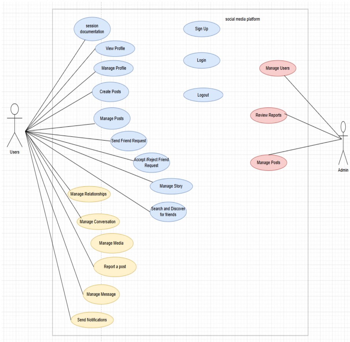
Figure 2.6: Use Case Diagram
